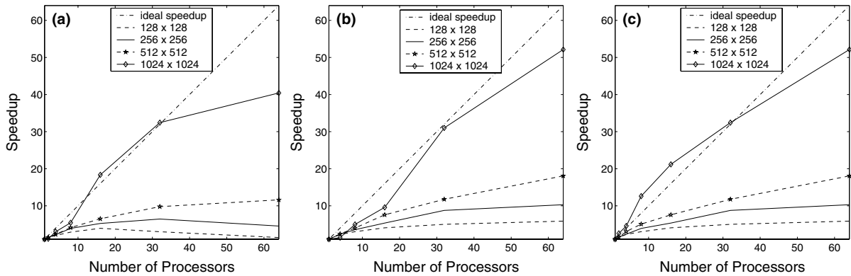
Fig. 2. The speedup of 2D Navier–Stokes code on SGI3800 with “2-n” scheme (a), “4-n” scheme (b), and “ideal” scheme. The values used in the “ideal” scheme are the top speedup among 1-n, 2-n, and 4-n schemes for the same resolutions and the same numbers of processors.
