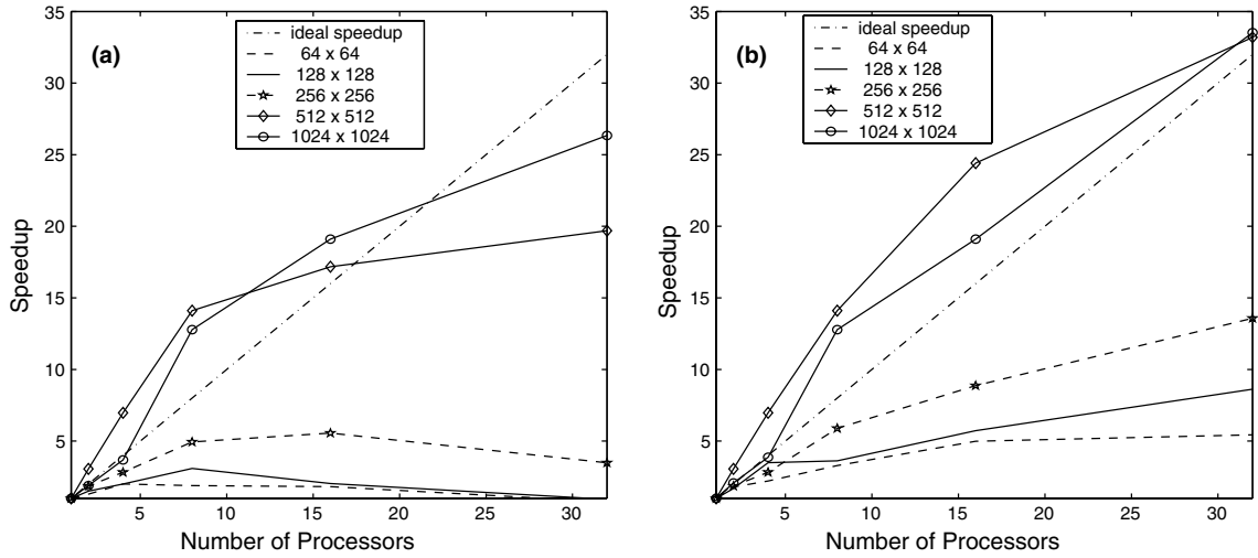
Fig. 4. The performance on SGI3800: (a) the speedup of 2D Boussinesq code with PFFFT scheme (or “1-N” scheme); (b) the speedup of 2D Boussinesq code with “ideal” scheme. The values used on (b) are the top speedup among 1-N, 2-N, 4-N, and 8-N schemes for the same resolutions and the same numbers of processors.
